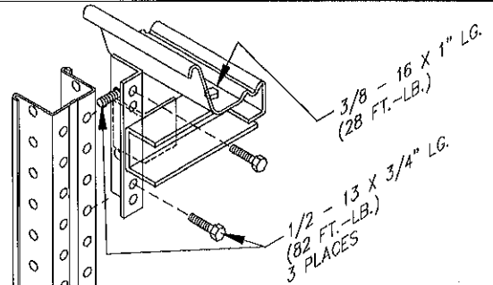
ALTERNATE ELL FOR ROLLED RAIL
