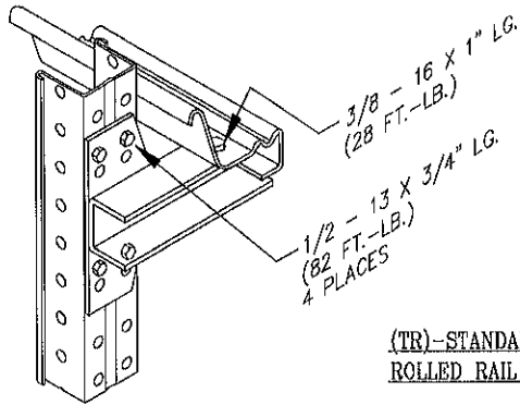
(LR)-STANDARD ELL FOR ROLLED RAIL
